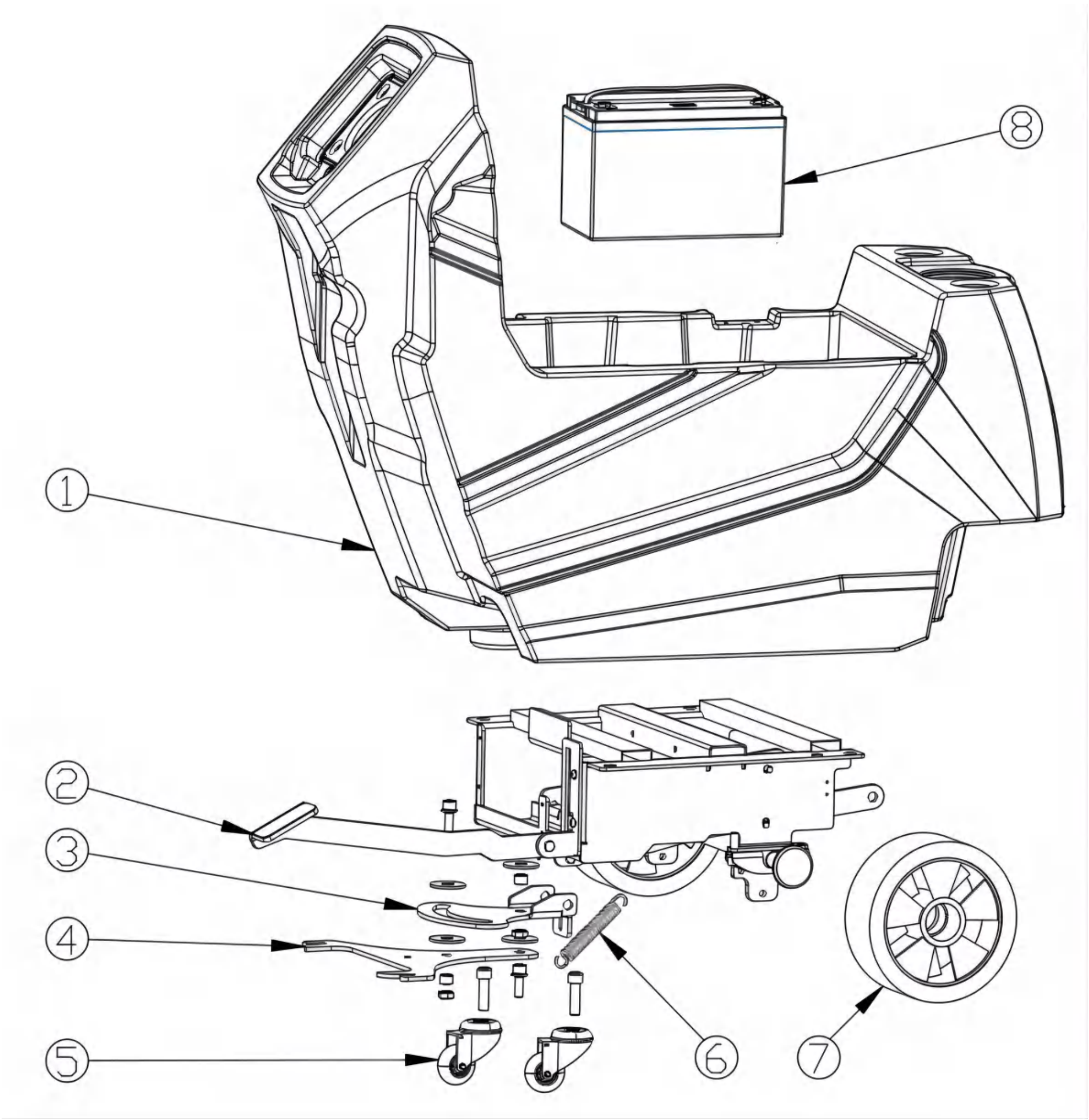
Fig. 4 -SOLUTION TANK GROUP
