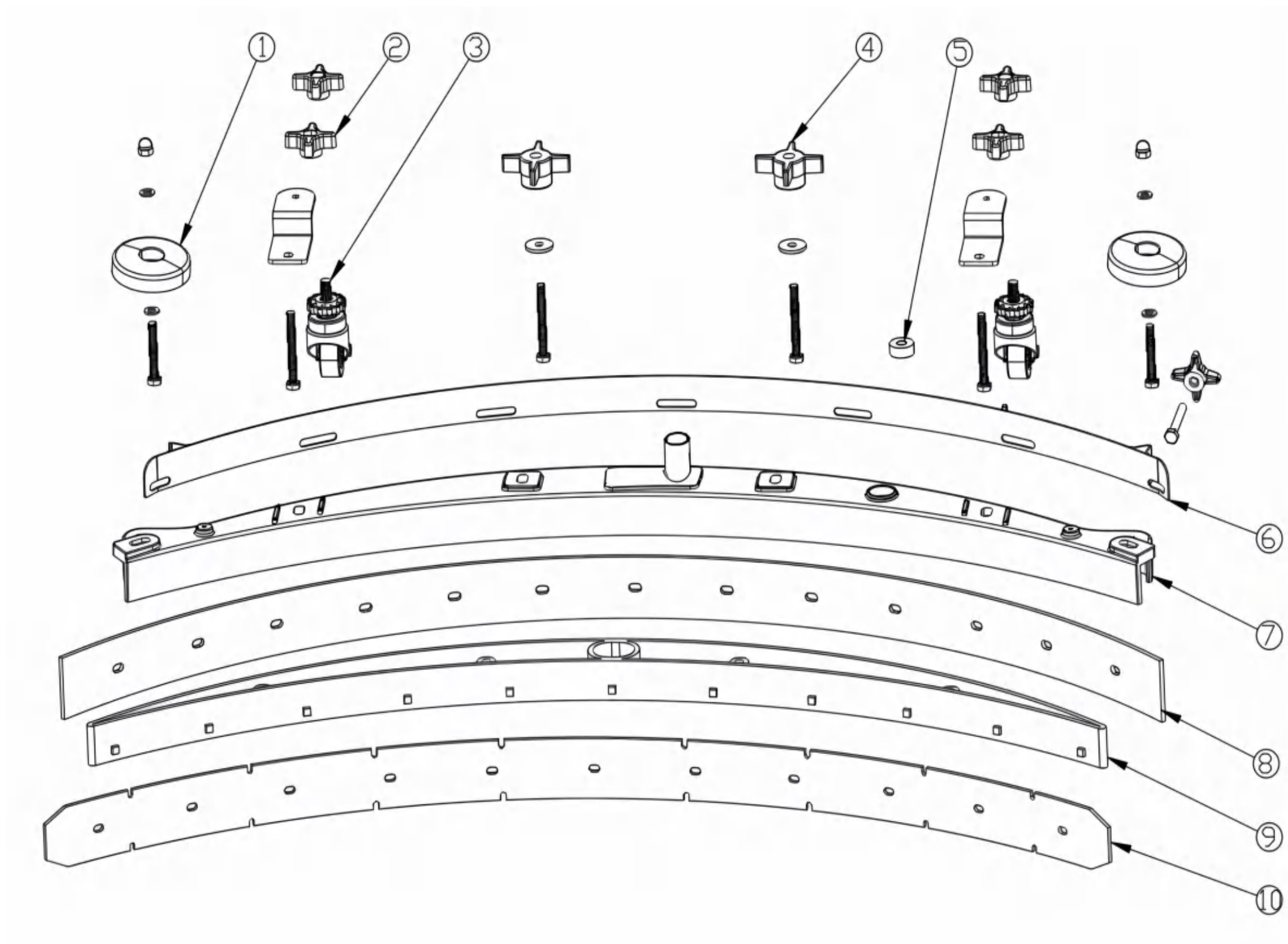
Fig. 8 -HOSE GROUP
