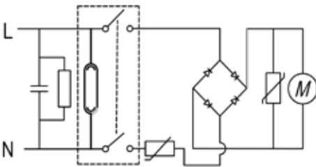
RSV 130 (DRW 20715) 120V 800W
