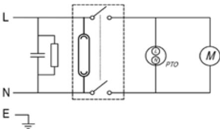
RSV 130 (DRW 20715) 120V 800W
