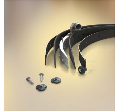
Vispa 35 E-B-BS In order to ensure excellent drying performance, the squeegee rubbers should be kept always clean. When worn out, they are very easy to replace
